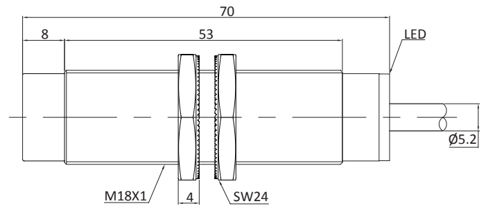
Fig. 4 Inductive sensor with cable (non-flush)
