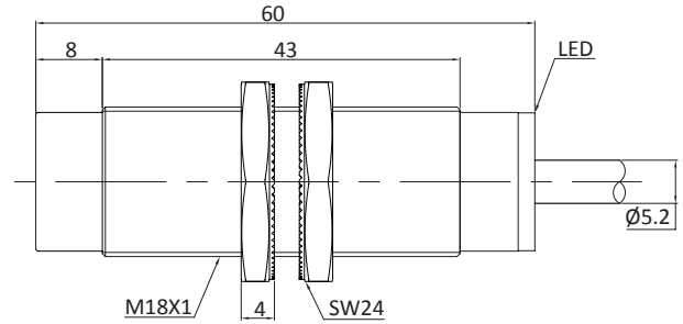
Fig. 2 Inductive sensor with cable (non-flush)
